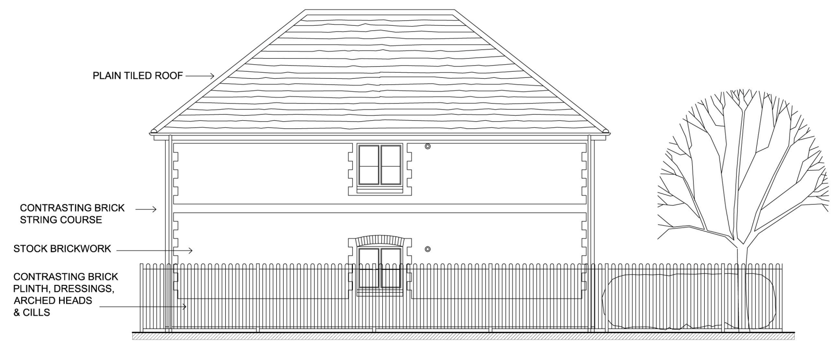
South Elevation
