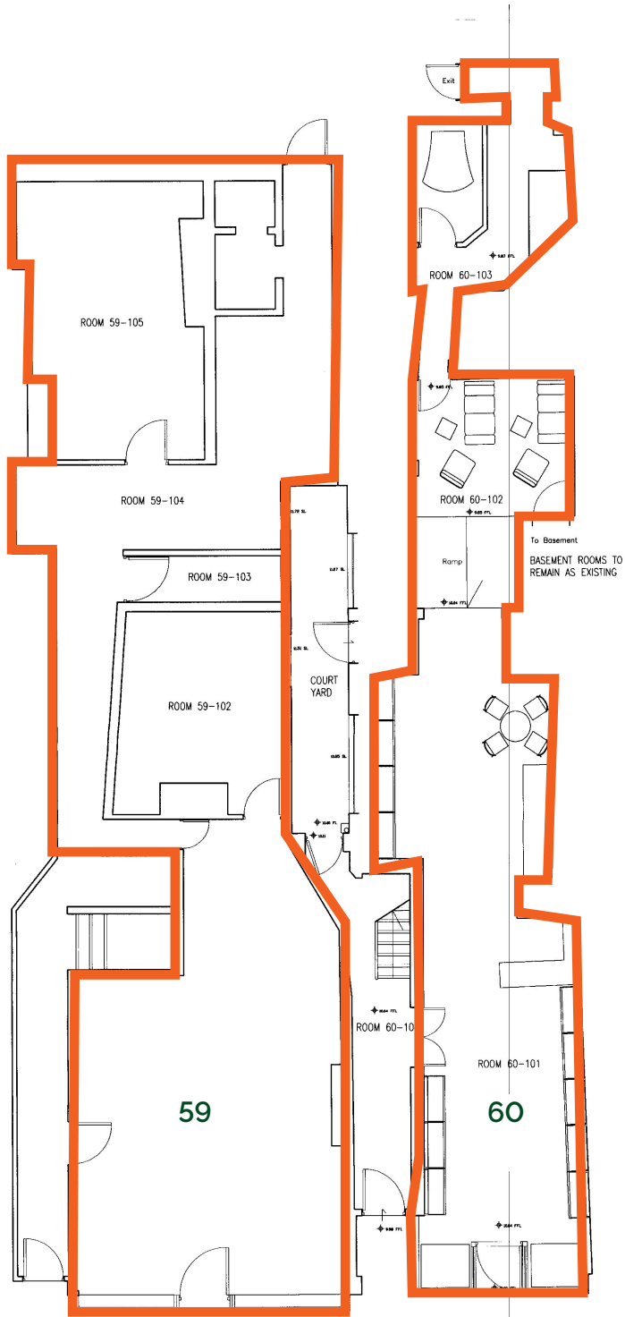
1 - 1:50@A1 GROUND FLOOR PLAN EXISTING
