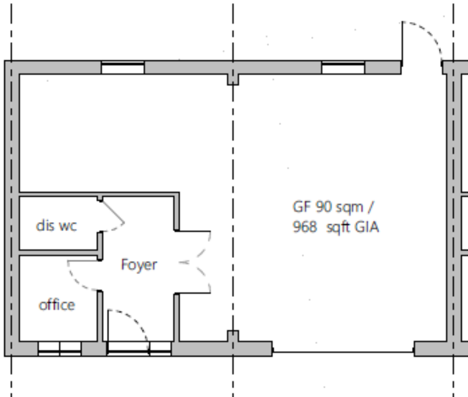
UNITS 1-8 TYPICAL GROUND FLOOR PLAN
