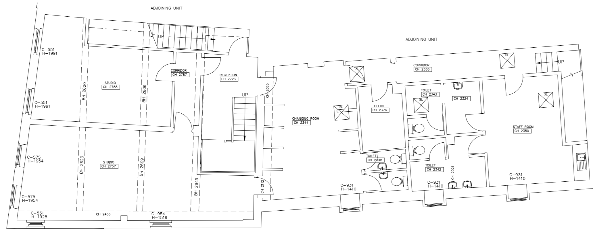
FIRST FLOOR
