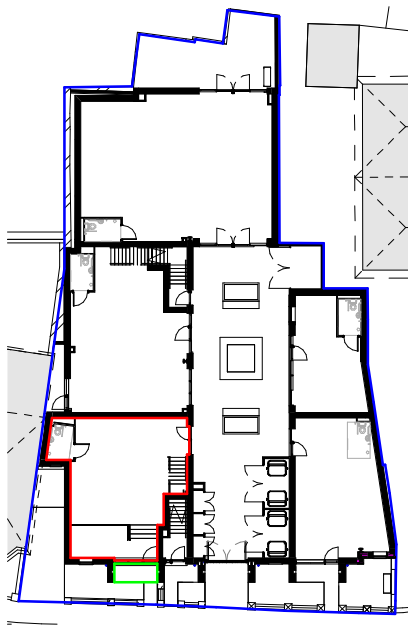
1 Ground Floor Block 1 : 500
