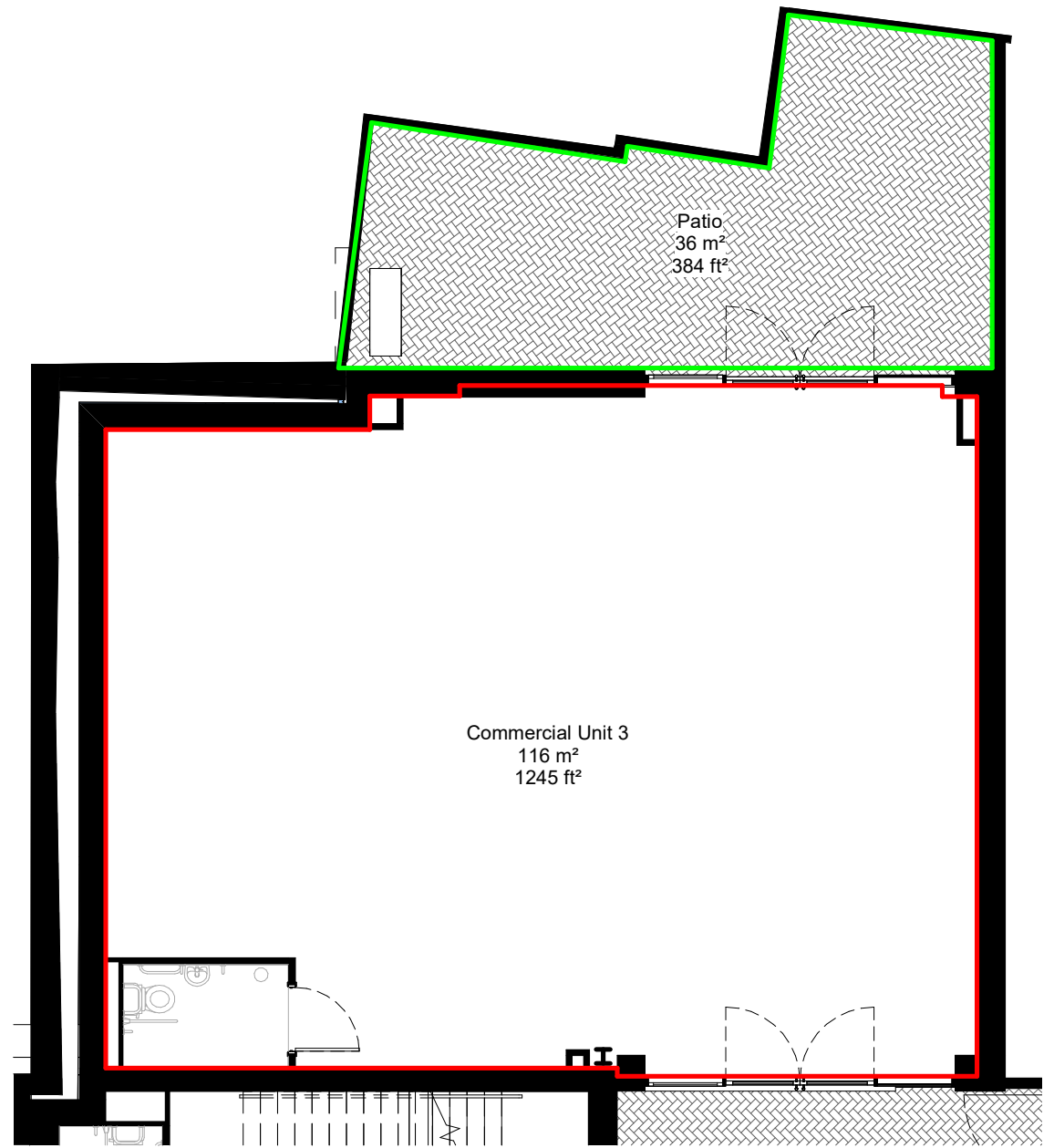
2 Commercial Unit 3 - Conveyance Pan 1 : 100
