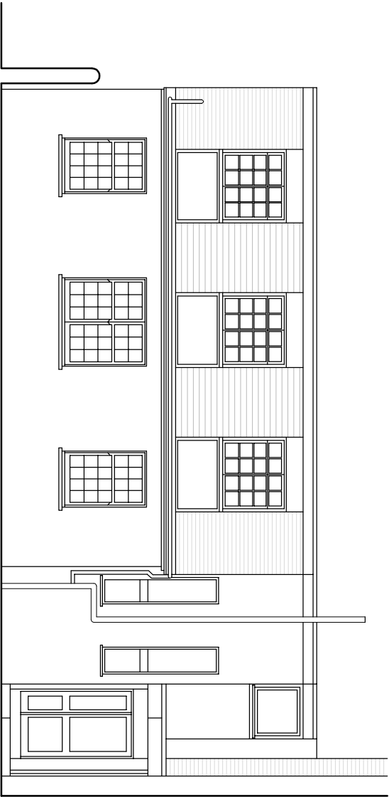
Front Elevation 1:100 As existing
