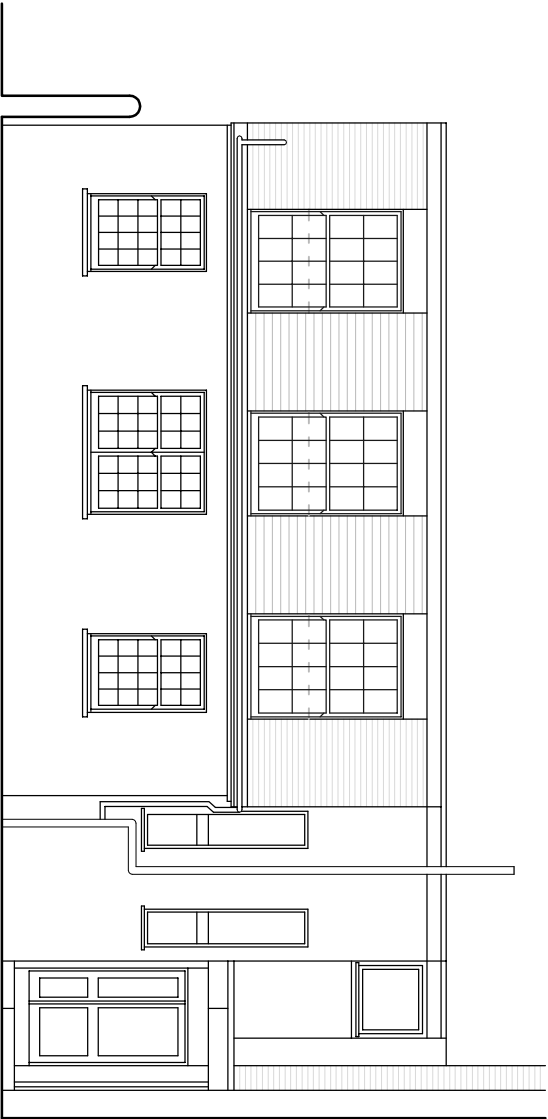
Front Elevation 1:100 As proposed
